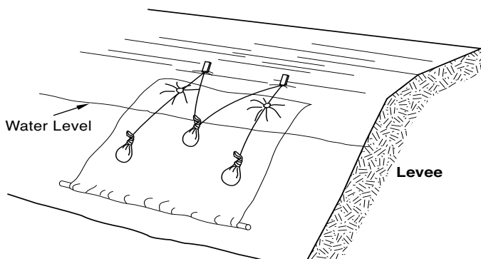
Figure 9: Waterside boil protection
